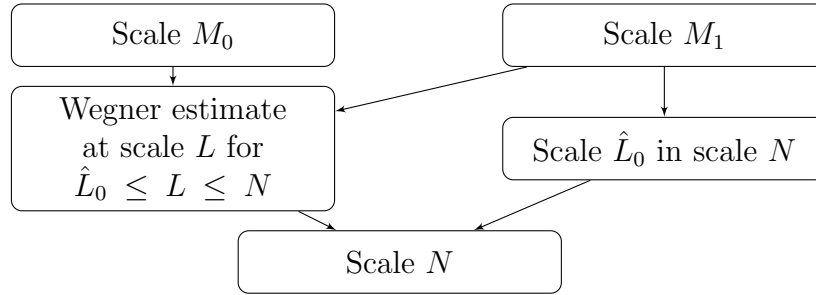
Figure 7.1: General outline of the proof
