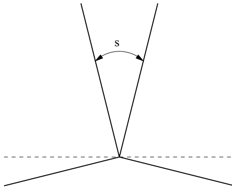
Figure 1. The region \tilde{A}_s
