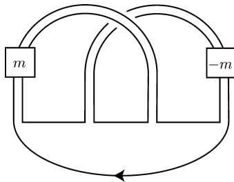
FIGURE 2.5. Negative amphichiral knots \mathbb{E}^m .
