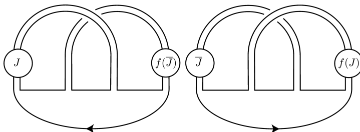
FIGURE 2.1. Families of negative amphichiral knots K .
