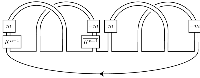
FIGURE 2.11. The examples K^n .
