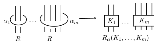
FIGURE 2.7. R_{\vec{\alpha}}(K_1, \dots, K_m) : infection of R by K_j along \alpha_j .
