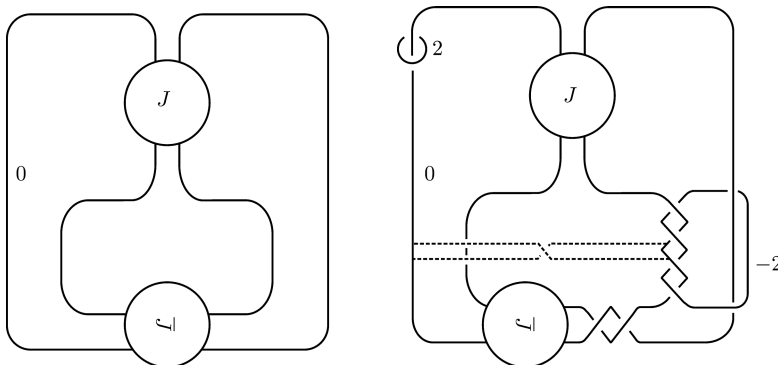
FIGURE 2.3. Adding a band.
