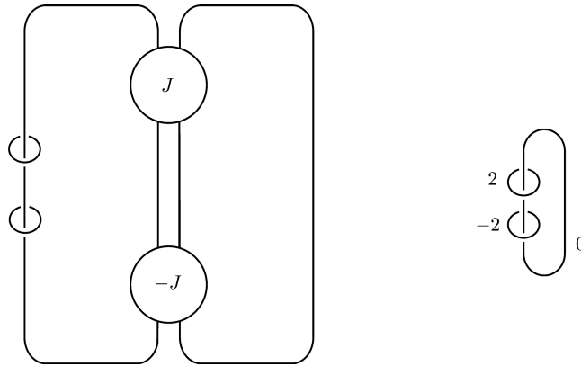
FIGURE 2.4. L_2 and L_4 .
