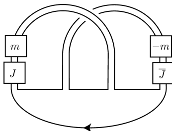
FIGURE 2.6. Families of negative amphichiral knots \mathbb{E}^m(J) .
