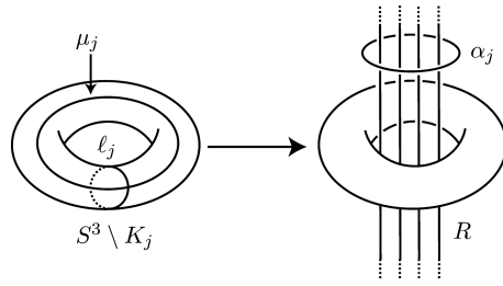
FIGURE 2.8. Infection as replacing a solid torus by a knot exterior.
