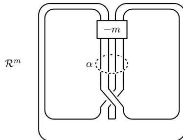
FIGURE 2.10. Doubling operators \mathcal{R}_\alpha^m .
