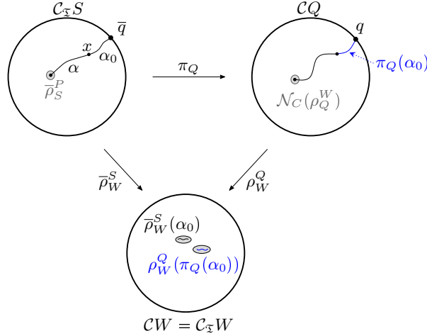
FIGURE 1. Proof of Lemma 4.18 when W \not\sqsubseteq Q .
