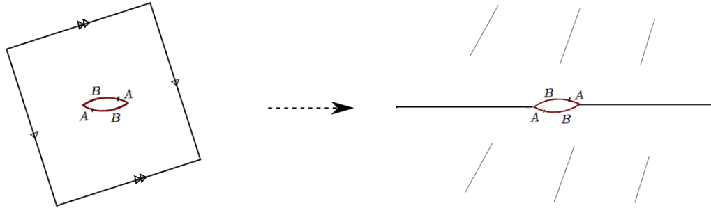
FIGURE 1. (An example of a half-plane structure.) The genus-2 surface (on the left) is obtained by an interval exchange on a slit of irrational slope on a flat torus. The corresponding Teichmüller ray “stretches” the singular-flat metric in the vertical direction. A half-plane differential of order 2 on a punctured torus (on the right) then arises as the Gromov-Hausdorff limit when basepoints are taken to lie on the critical graph.
