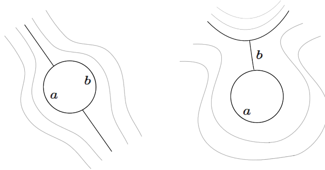
FIGURE 4. A 2-planar end has two possible patterns of metric spines. The non-negative edge lengths (a, b) for each pattern parametrize cells that fit together to form \mathbb{R}^2 . (See Propn. 3.3.)
