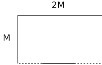
FIGURE 10. For large M the extremal length of the family of arcs between the arcs shown in bold is \sim 2 \ln M + D for some real (universal) constant D . A truncated k -planar end is a k -fold branched cover of this.
